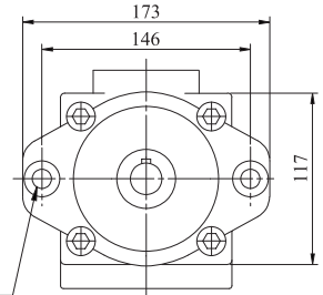
2-Ø 13.5 HOLES Ø 25 SPOTFACE 1 DEEP
