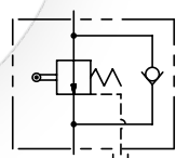
常閉 Normally Closed CLG/CLT
