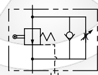
常開 Normally Open CLG/CLT
